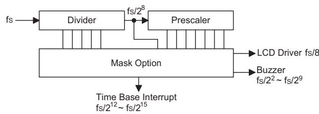
Time Base
