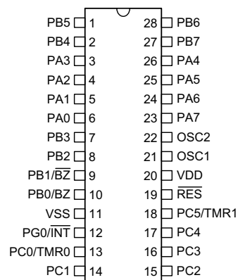
HT48E50 – 28 SKDIP-A/SOP-A
