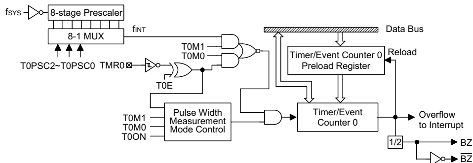
Timer/Event Counter 0
