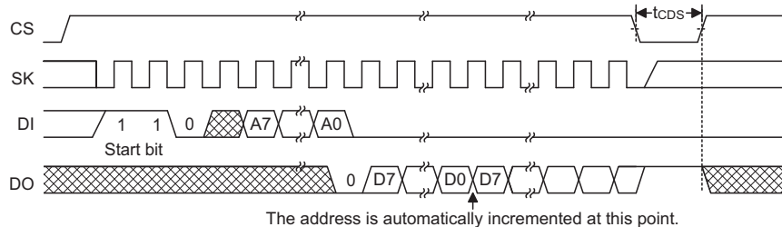
READ Timing
