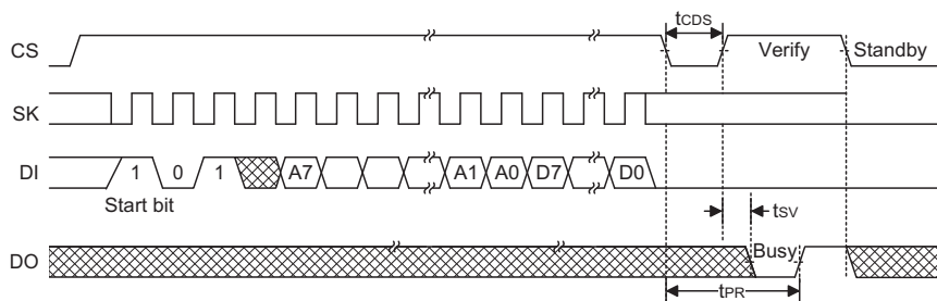
WRITE Timing
