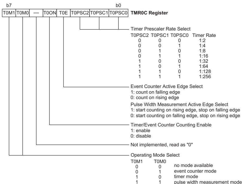
Timer/Event Counter 0 Control Register
