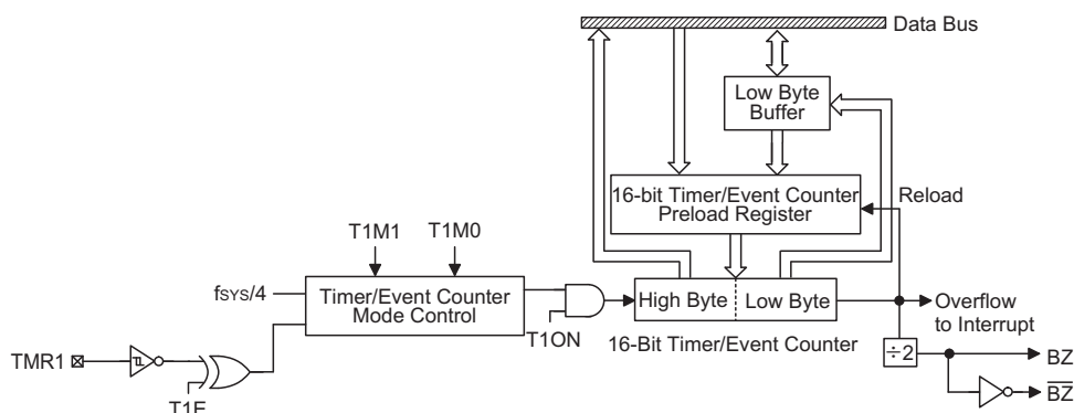
16-bit Timer/Event Counter Structure
