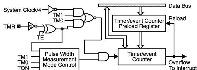
Timer/event counter
