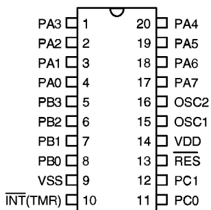
HT48R31-1/HT48R31-2 - 20 DIP-F-0
