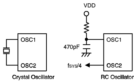
System oscillator
