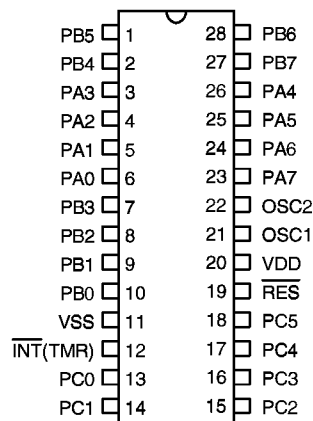
HT48R31-1/HT48R31-2 - 28 SKDIP-B-0
