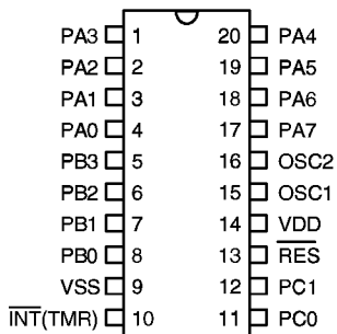
HT48R31-1/HT48R31-2 - 20 DIP-F-0
