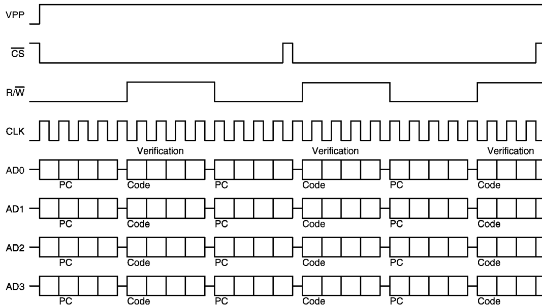
Non-successive verification
