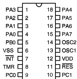
HT48R31-1/HT48R31-2 - 18 DIP-A-0
