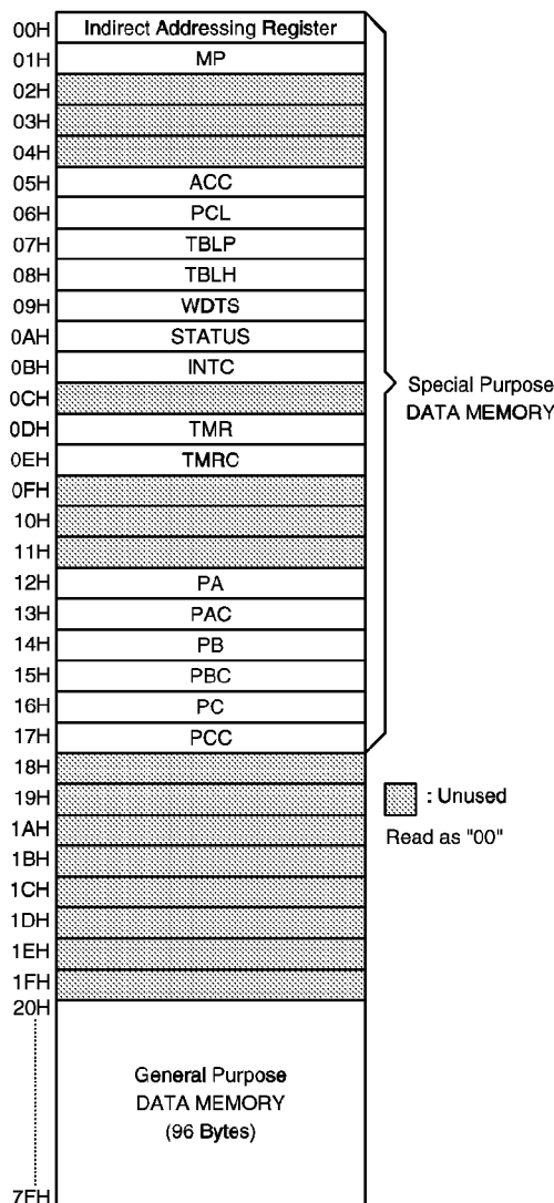
RAM mapping
