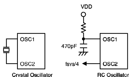
System oscillator
