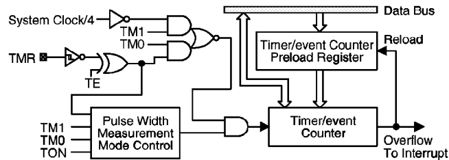
Timer/event counter
