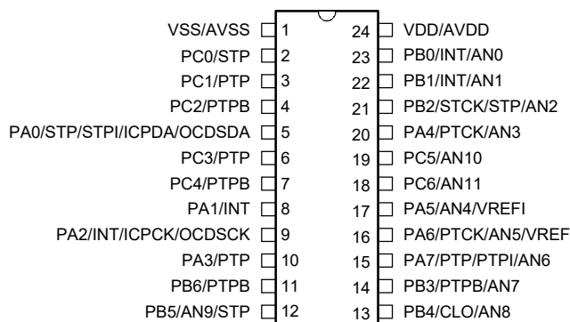
HT66F3194/HT66V3194 24 SSOP-A
