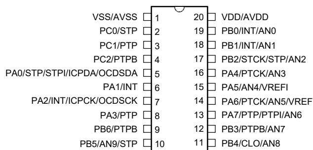
HT66F3194/HT66V3194 20 NSOP-A
