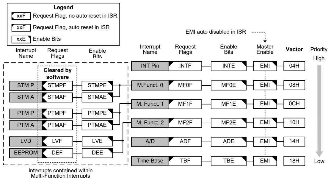
Interrupt Structure
