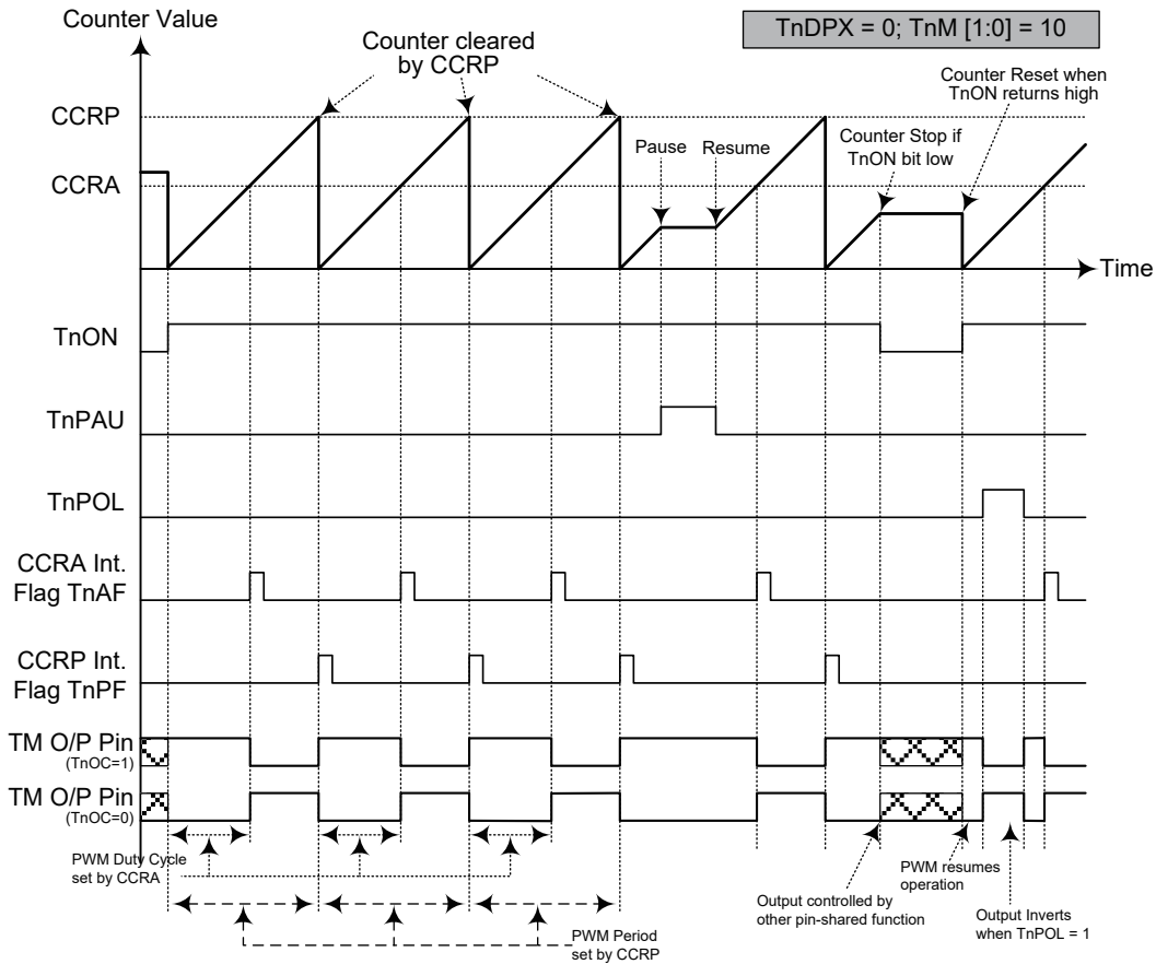
PWM Mode – TnDPX=0
