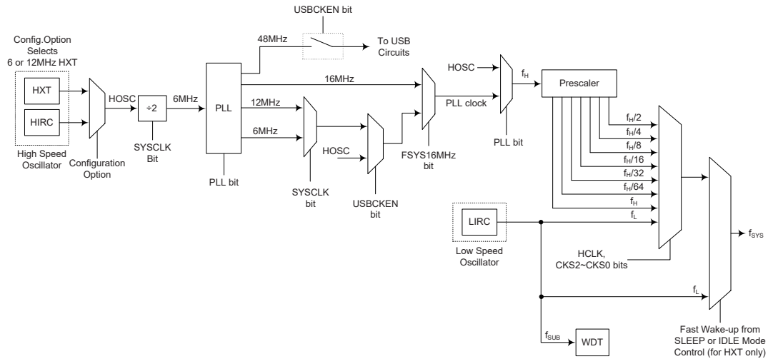
Device Clock Configurations – HT66FB542
