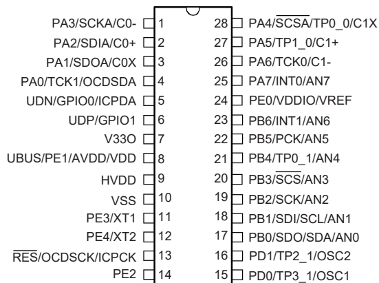
HT66FB550/HT66VB550 28 SSOP-A
