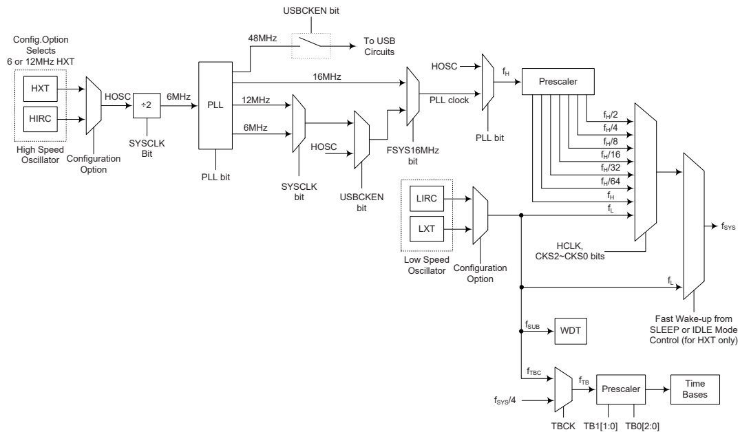
Device Clock Configurations – HT66FB540/HT66FB550/HT66FB560
