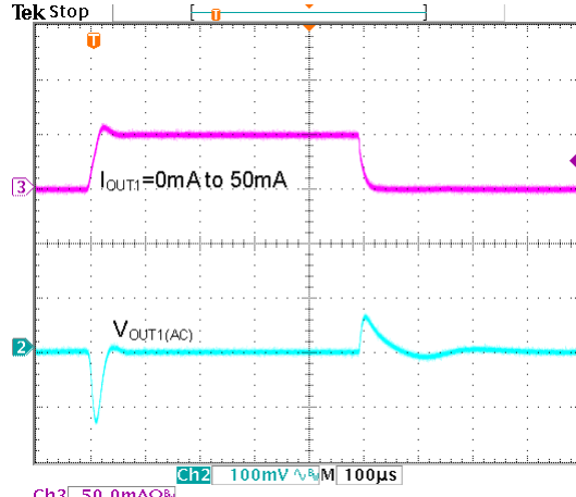
HT72D5015 V OUT1 =5.0V V IN =6.0V C IN =C OUT1 =1 \mu F V EN1 =V IN V EN2 =0V
