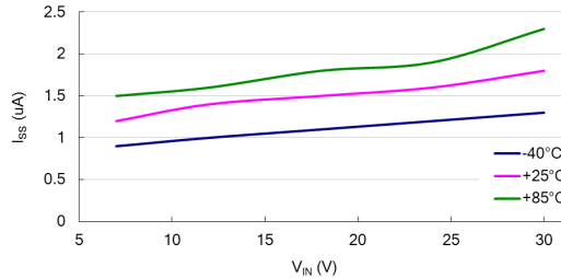
I SS vs V IN : HT7350-2 (I OUT =0mA)
