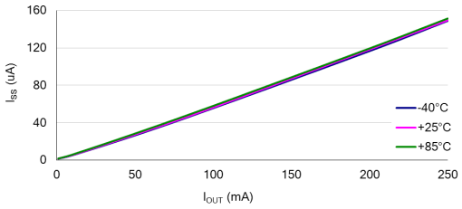
I SS vs I OUT : HT7333-2 (V IN =5.3V)
