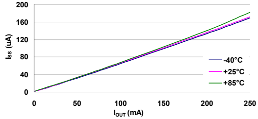
I SS vs I OUT : HT7350-2 (V IN =7.0V)
