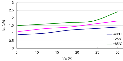
I SS vs V IN : HT7333-2 (I OUT =0mA)
