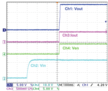
Enable ON (HT7463A, I_{OUT}=500mA )
