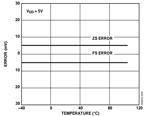
Figure 9. Zero-Scale Error and Full-Scale Error vs. Temperature
