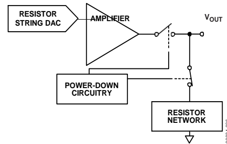
Figure 27. Output Stage During Power-Down
