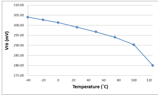
Fig.2 Feedback Voltage VS Temperature
