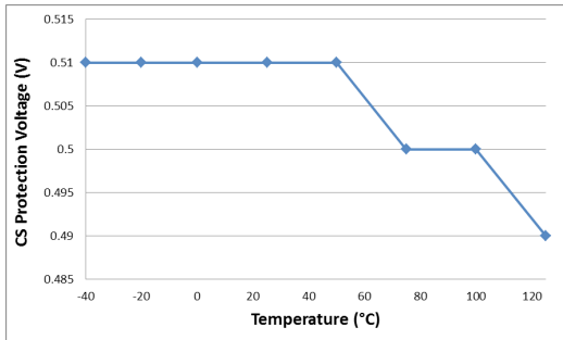
Fig.3 CS Protection Voltage VS Temperature
