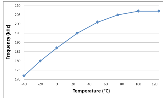
Fig.5 Frequency VS Temperature
