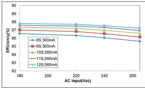
Figure 9. Efficiency vs. AC Voltage
