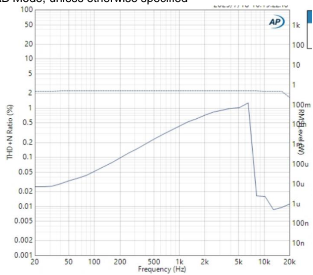
frequency vs THD+N, P_o \approx 0.5W
