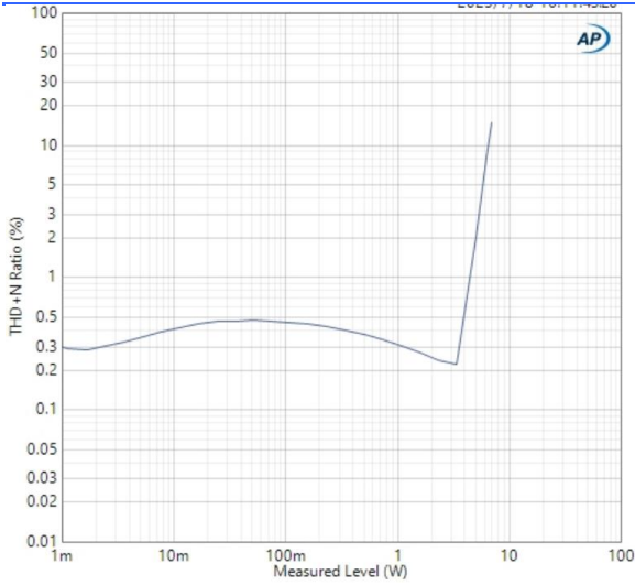
Output power vs THD+N, f = 1kHz
