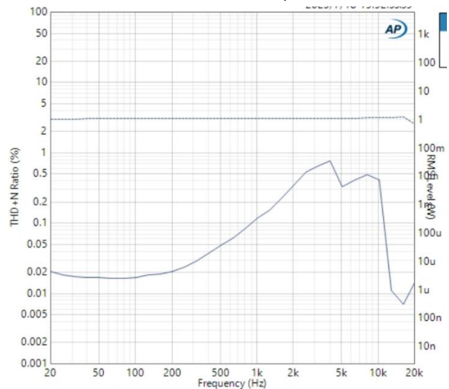
frequency vs THD+N, P_o \approx 1W
