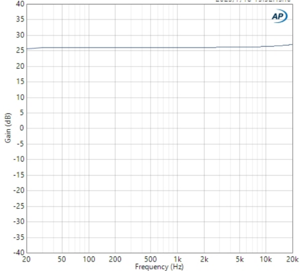
Frequency Respond C_{IN}=1\mu F , R_{IN} = 20k
