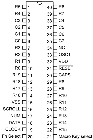
HT82K628A - 40 DIP
