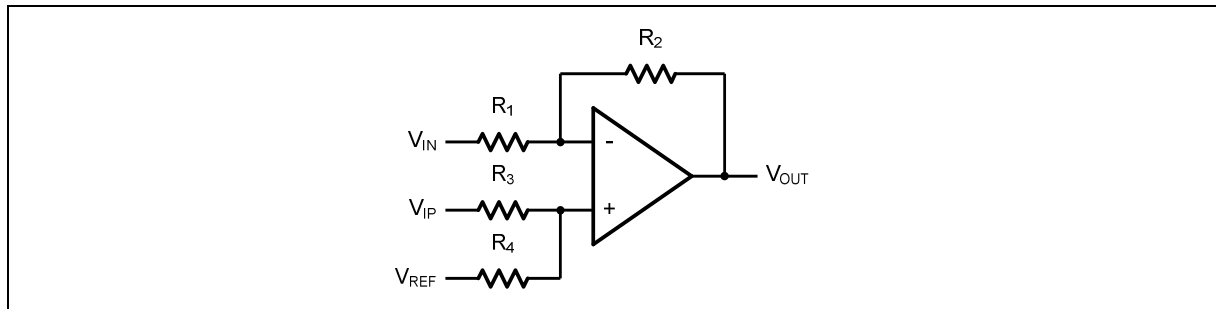
Figure 4. Differential Amplifier
