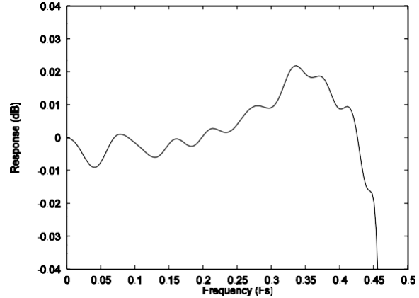
Figure 30 ADC Digital Filter Ripple – Type 0
