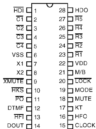
HT9245-1DL – 28 DIP
