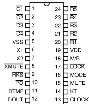
HT9245-1CL – 24 DIP
