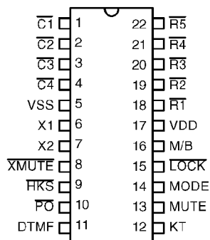
HT9245-1AL – 22 DIP
