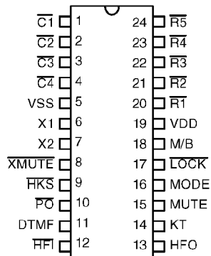
HT9245-1BL – 24 DIP
