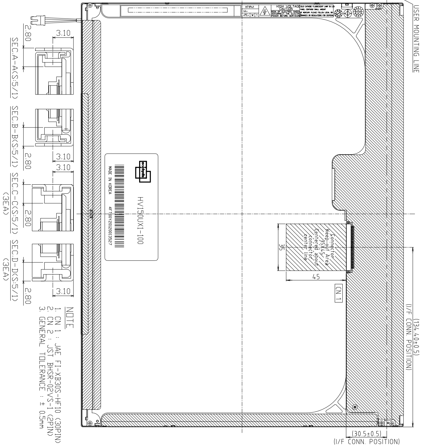
Figure 6. TFT-LCD Module Outline Dimensions (Rear view)
