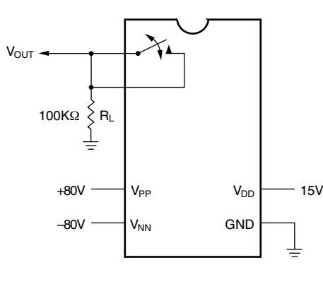
DC Offset ON/OFF
