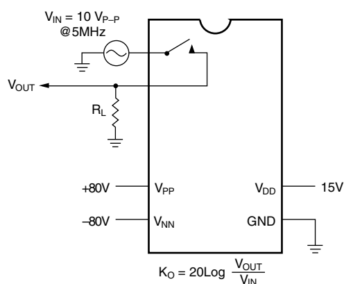
OFF Isolation
