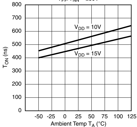
T_{ON} vs. Ambient Temp V_{PP}/V_{NN} = \pm 80V
