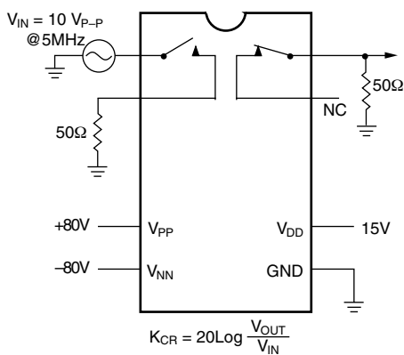
Crosstalk
