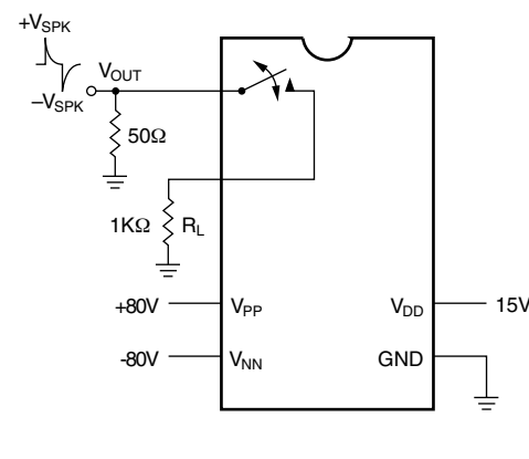
Output Voltage Spike
