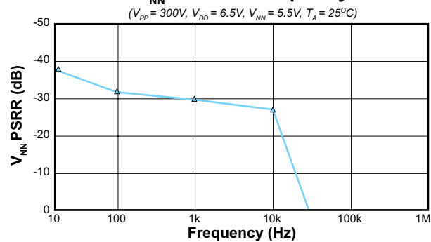
V_{NN} PSRR vs Frequency
