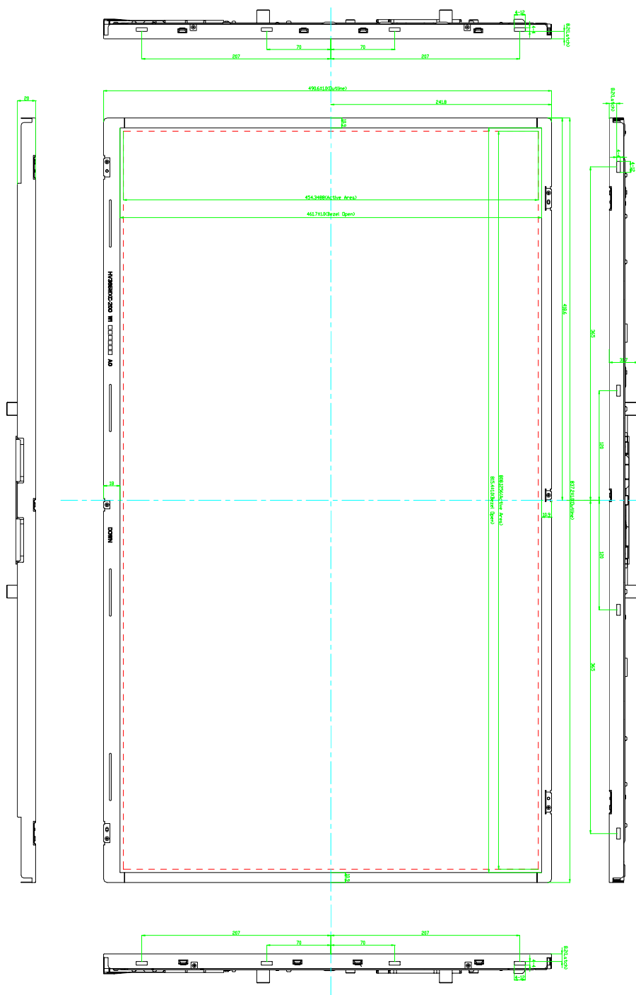
< Figure 4. TFT-LCD Module Outline Dimensions (Front View) >
