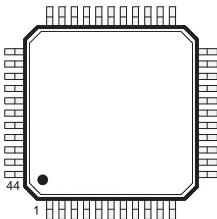
44-Lead PQFP
