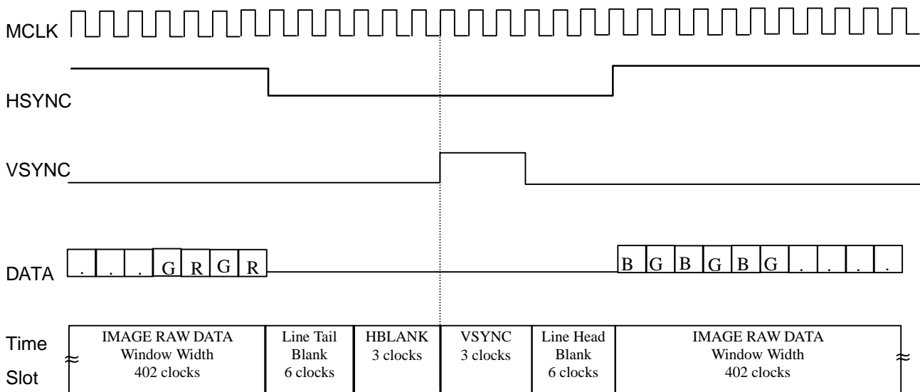
Fig.3 Odd Line Data Timing
