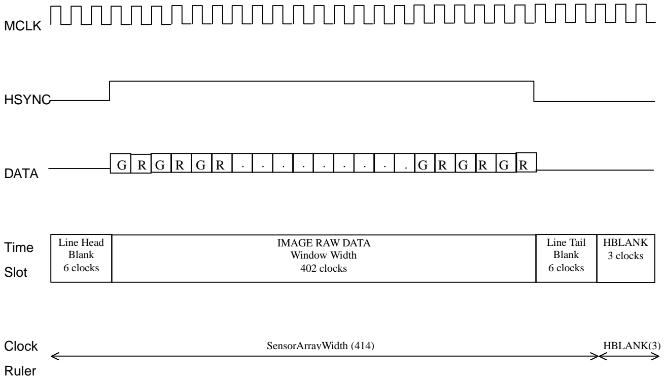
Fig.3 Odd Line Data Timing
