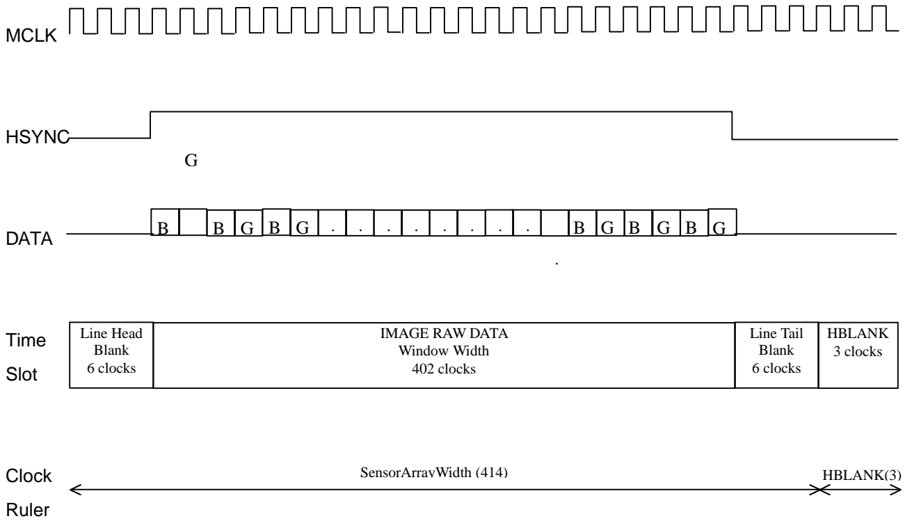
Fig.6 Even Line Data Timing
