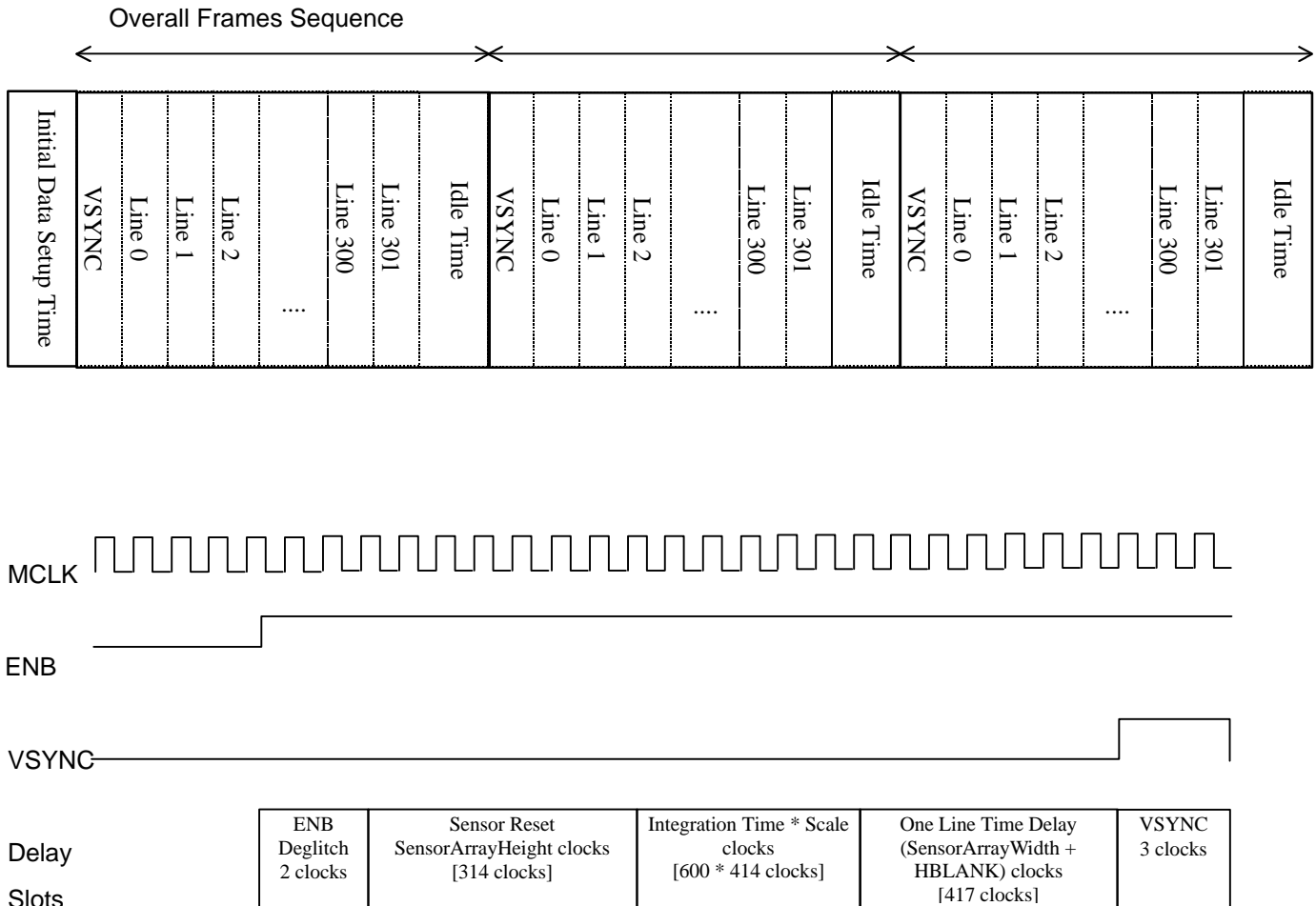
Fig. 5 Initial Data Setup Time after ENB gets active
