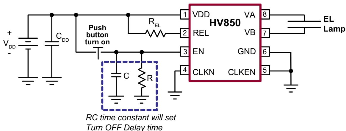
Figure 2: Push Button Turn on with Delay Turn off (For V_{DD} = 3.4V to 4.2V only)
