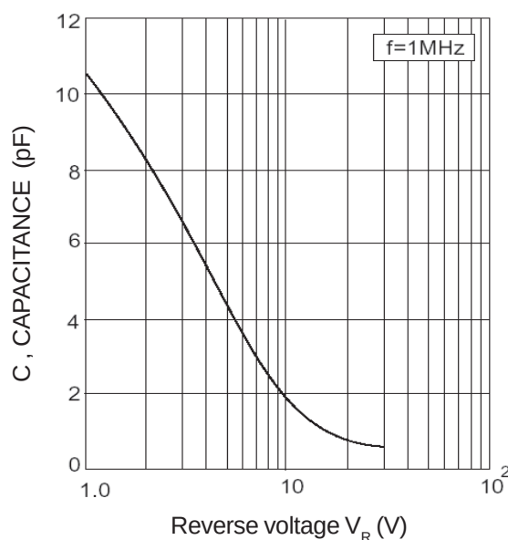
Fig.2 Capacitance Vs. Reverse voltage
