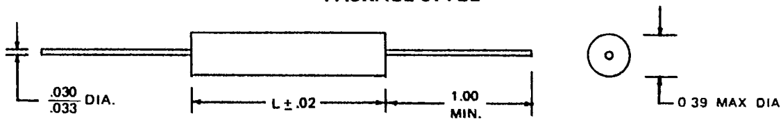
FIG. 3 PACKAGE STYLE
