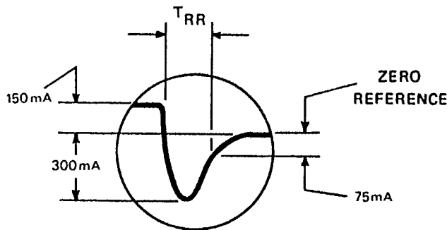
TYPICAL REVERSE RECOVERY WAVEFORM
