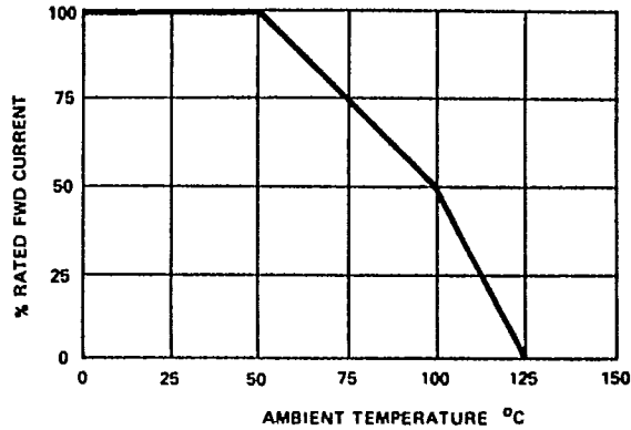
FIG. 1 OUTPUT CURRENT vs. AMBIENT TEMPERATURE
