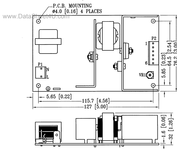
PCB FORMAT
