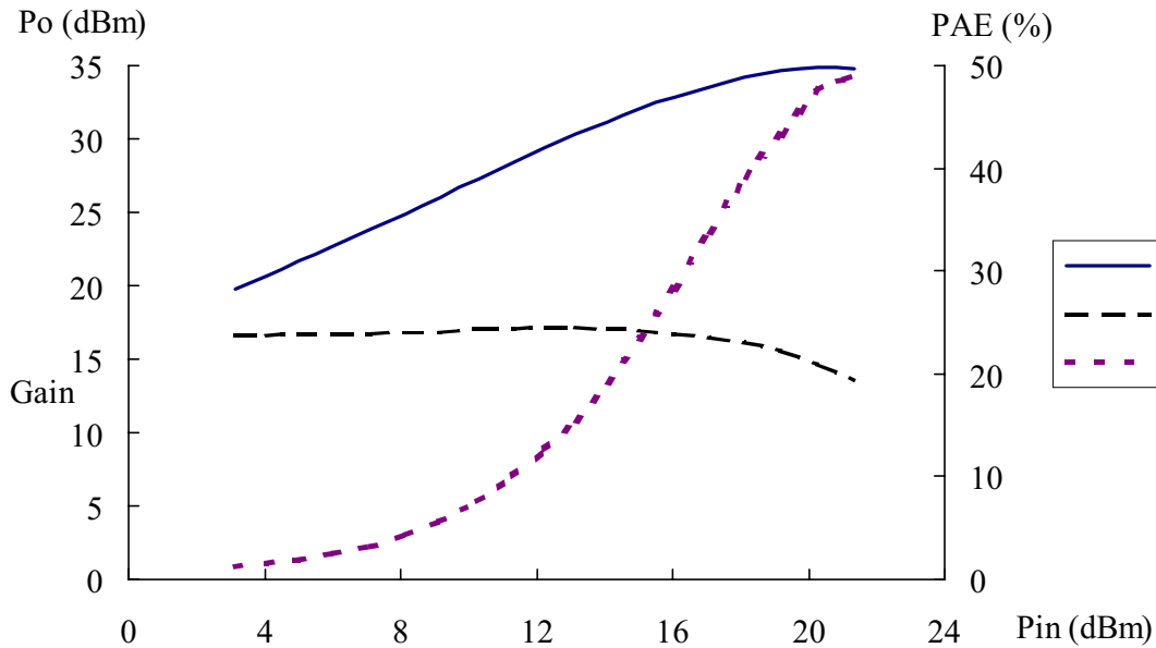
Output Power & Efficiency & Gain vs Input Power @ f=1.9 GHz, V_{ds}=10 V, I_{ds} = 0.5 I_{dss}
