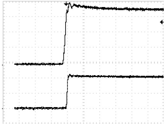
Start –up from Shutdown (1.00V/div 1.00V/div 100 \mu s/div)
