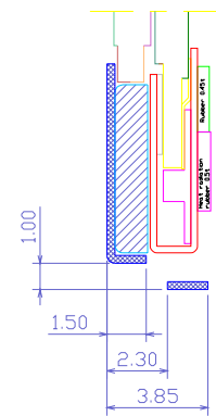
SECTION E-E(S:5/1)
