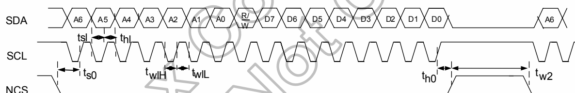
Figure 5.1 3 wire SPI Timing
