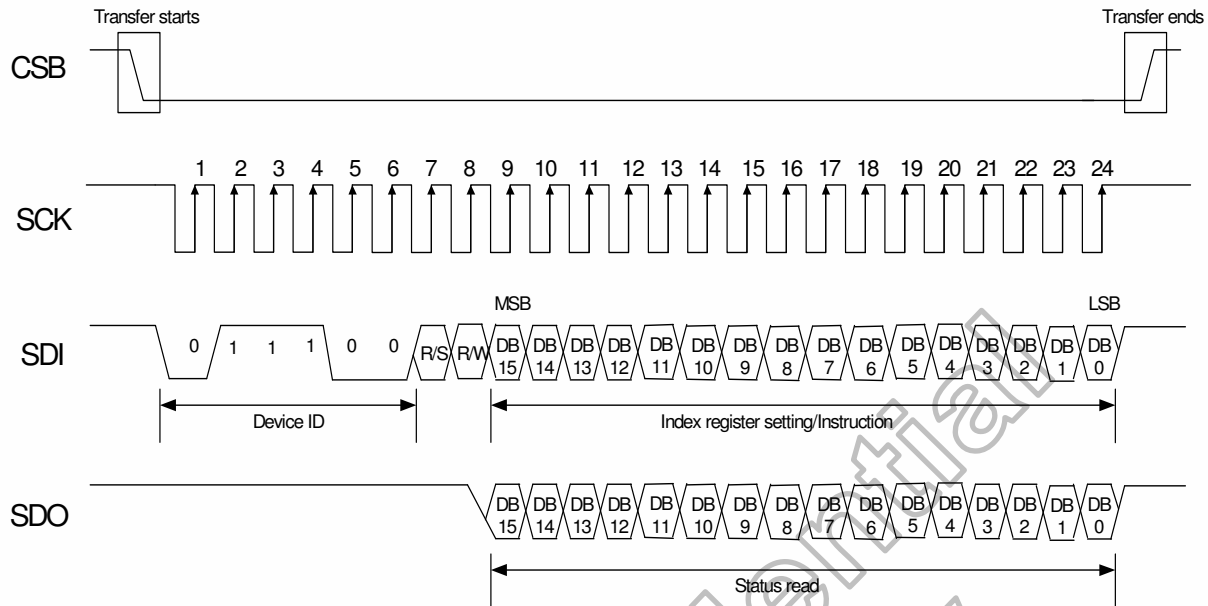
Figure 6. 1 SPI Timing
