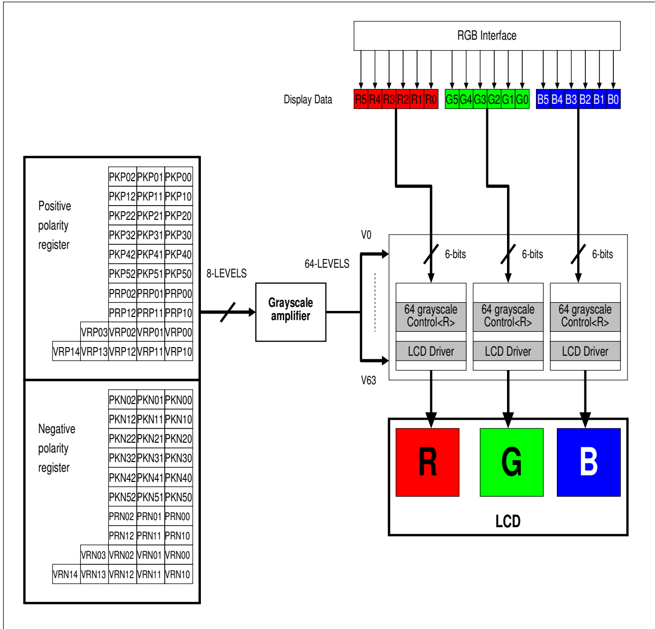
Figure 10. 1 Grayscale Control Block
