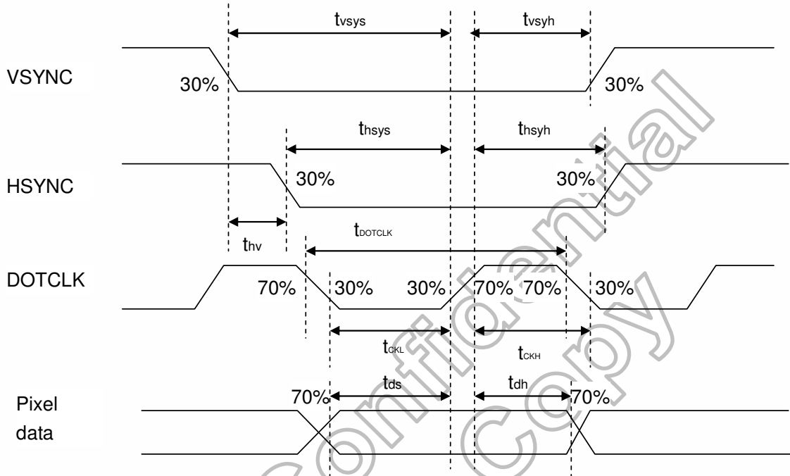
Figure13. 1 Pixel Timing
