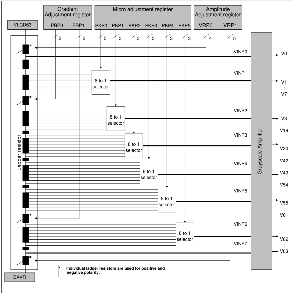
Figure 10. 2 Grayscale Amplifier
