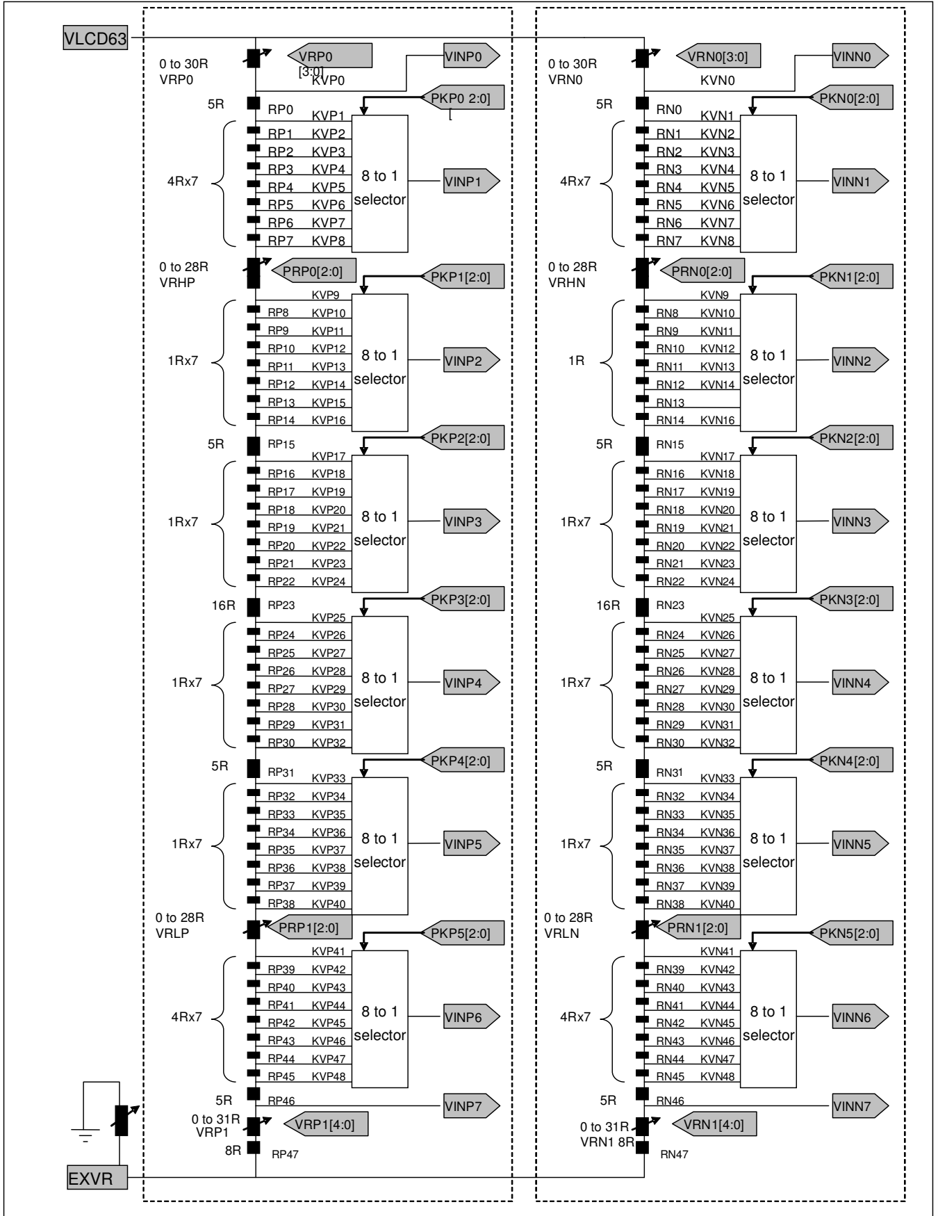
Figure 10. 3 Resistor Ladder for Gamma Voltages Generation
