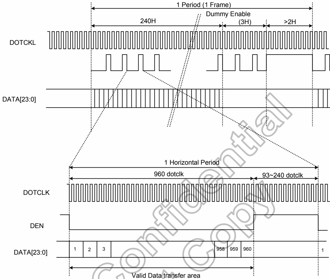
Figure13. 5 Data Transaction Timing in Serial RGB (8 bit) Interface (DE Mode)
