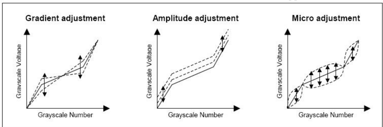
Figure 10. 4 Gamma Adjustment Function
