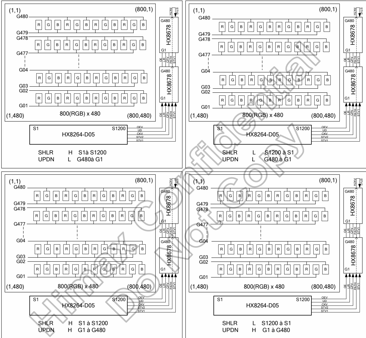
Figure 3. 7: HX8264-D05 Dual Gate 800(RGB) x 480 Application Block Diagram-2
