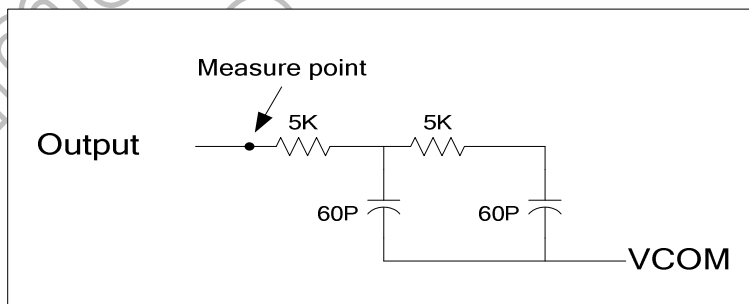
Figure 12. 3: Output Load Condition
