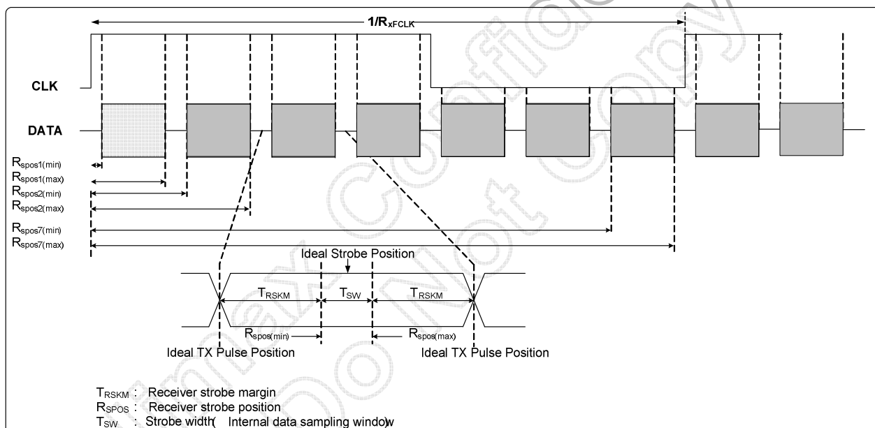
Figure 10.1: LVDS figure
