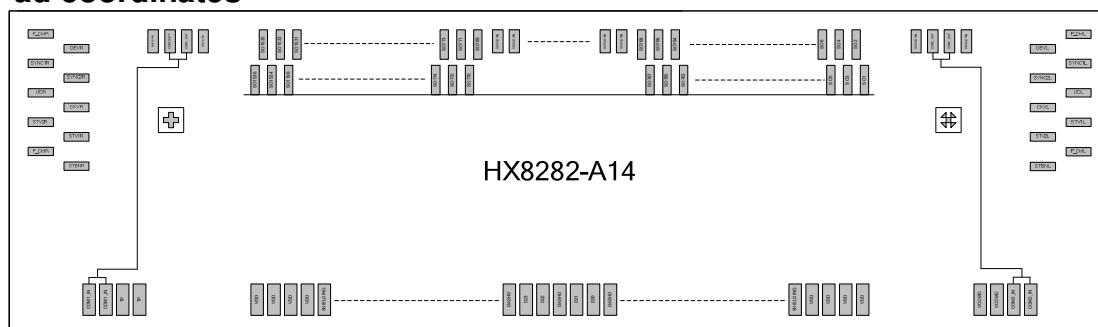
Figure 12.4: Pad coordinate
