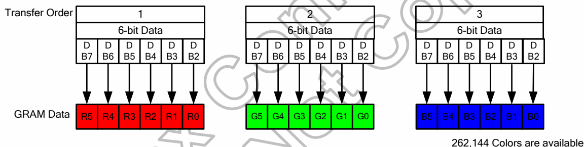
Figure 4-23: Input data bus and GRAM data mapping in 8-bit bus system interface with 18-bit-data input ( R17H=06h and "IM3, IM2, IM1, IM0"="0001")
