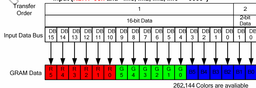
Figure 4-10: Input data bus and GRAM data mapping in 16-bit bus system interface with 18(16+2) bit-data input ( R17H=07h and "IM3, IM2, IM1, IM0"="0000")
