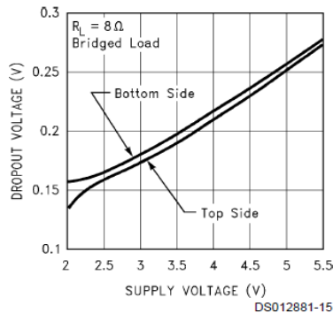
Dropout Voltage vs Supply Voltage
