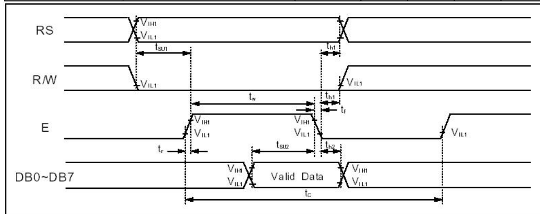
Figure 3 . Write Mode Timing Diagram
