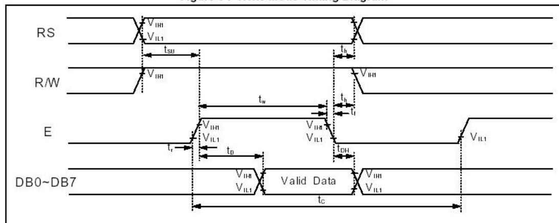
Figure 4 . Read Mode Timing Diagram
