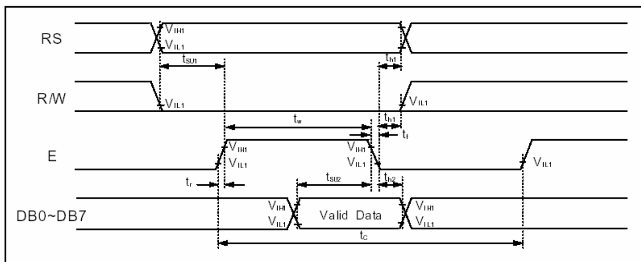
Figure 6 . Write Mode Timing Diagram
