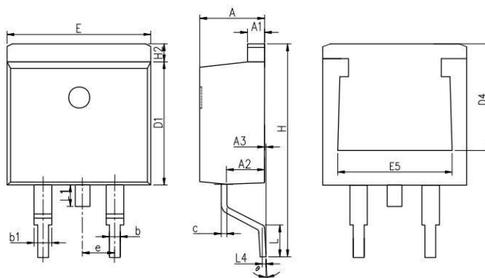
COMMON DIMENSIONS
