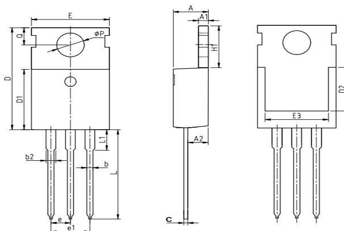
COMMON DIMENSIONS
