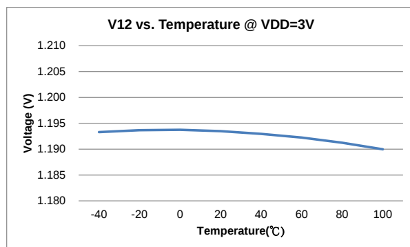
Figure V12 vs. Temperature
