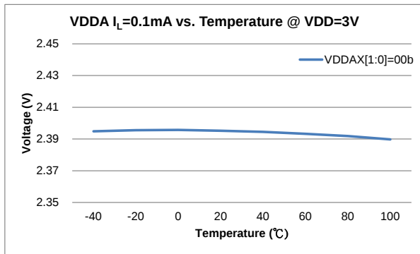
Figure VDDA vs. Temperature
