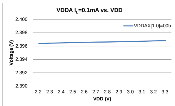
Figure VDDA vs. VDD
