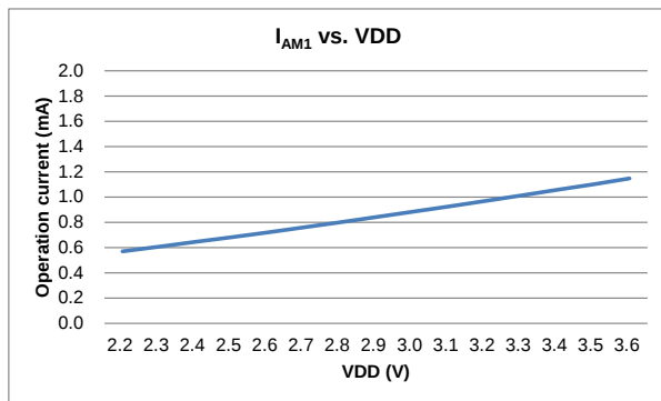
Figure I AM1 vs. VDD
