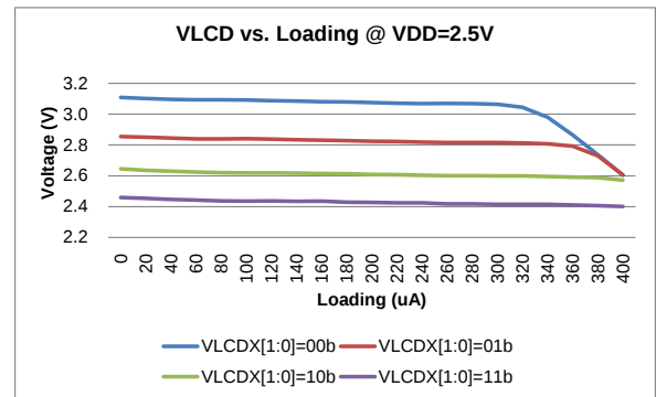
Figure VLCD vs. Loading
