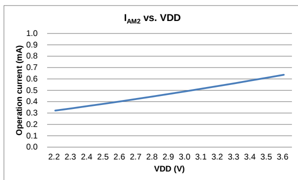
Figure I AM2 vs. VDD
