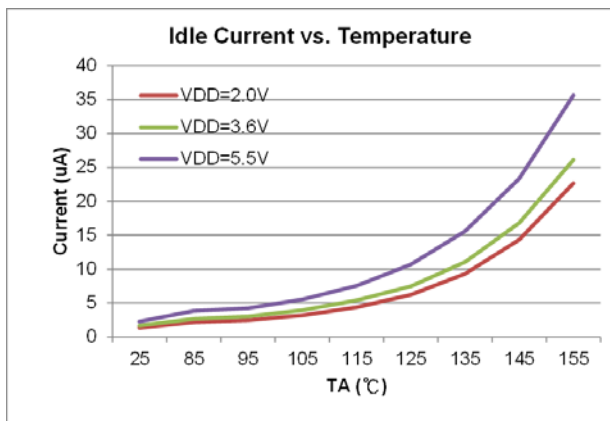
Figure 5.7-3 LP2 vs. Temperature
