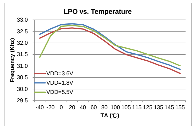
Figure 5.6-2 LPO Frequency vs. Temperature
