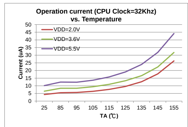
Figure 5.7-2 LP1 vs. Temperature
