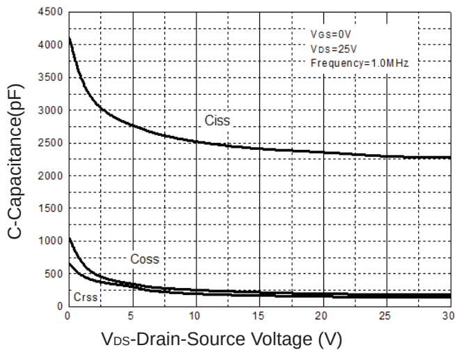
Figure 9: Capacitance Characteristics
