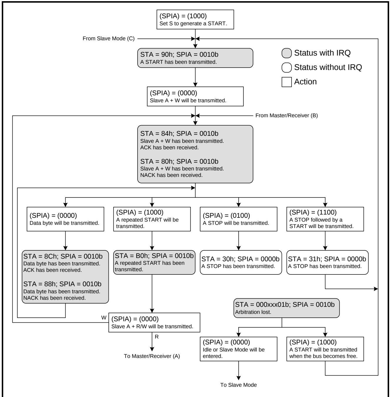
16-5 Master Transmitter Mode
