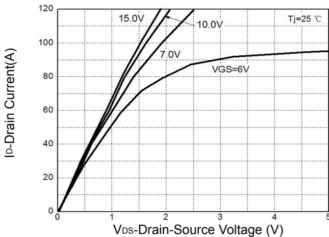
Figure 5: Output Characteristics
