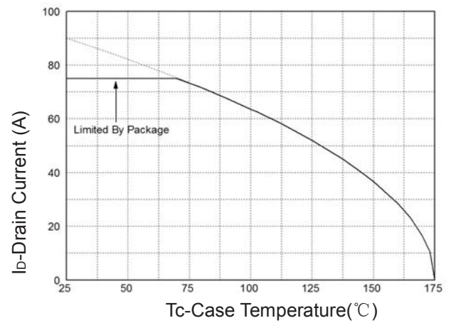
Figure 2: Drain Current
