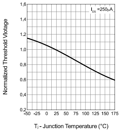
Gate Threshold Voltage
