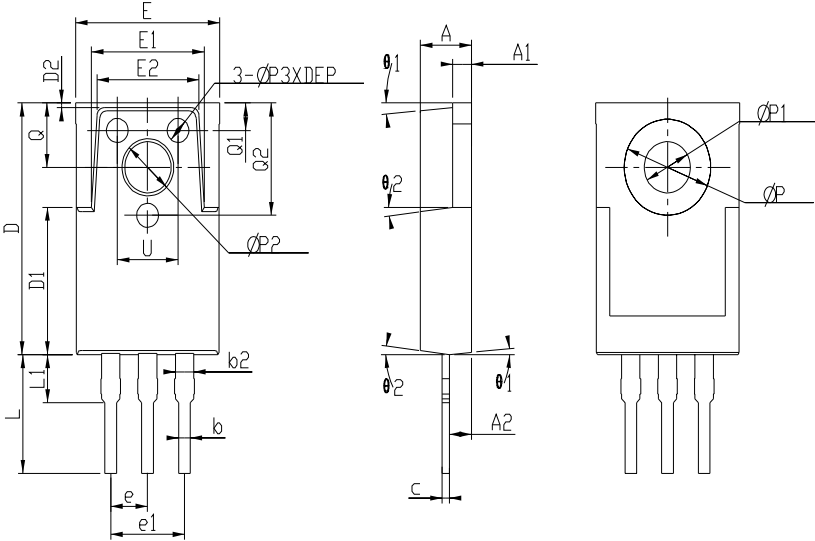
COMMON DIMENSIONS
