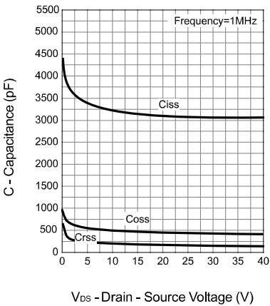
Capacitance
