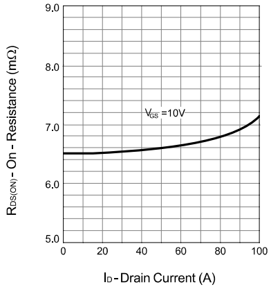
Drain-Source On Resistance
