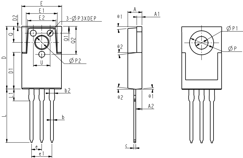
COMMON DIMENSIONS
