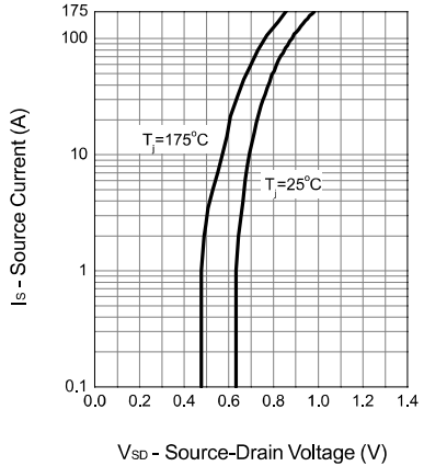
Source-Drain Diode Forward
