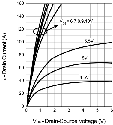
Output Characteristics
