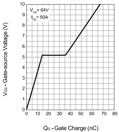
Gate Charge
