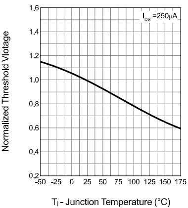
Gate Threshold Voltage
