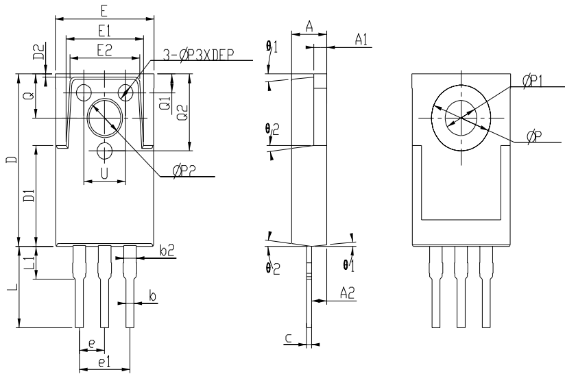
COMMON DIMENSIONS
