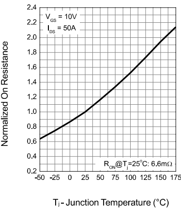
Drain-Source On Resistance
