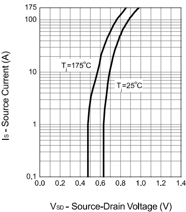
Source-Drain Diode Forward
