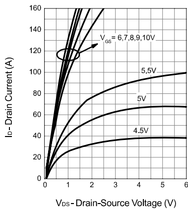
Output Characteristics
