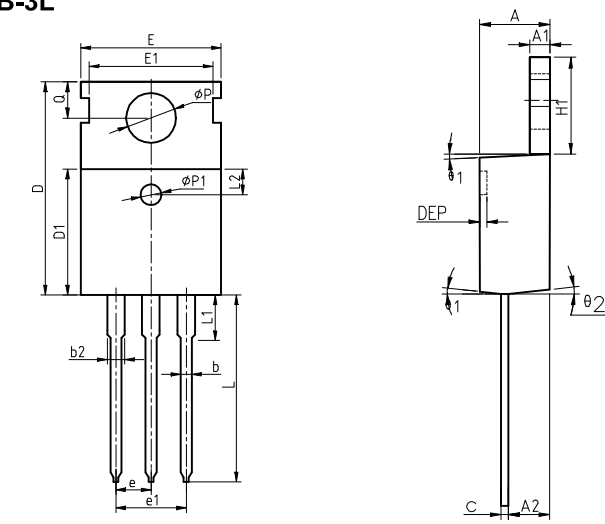
COMMON DIMENSIONS
