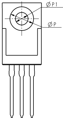
COMMON DIMENSIONS
