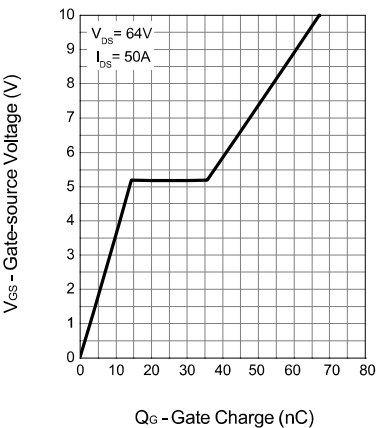
Gate Charge
