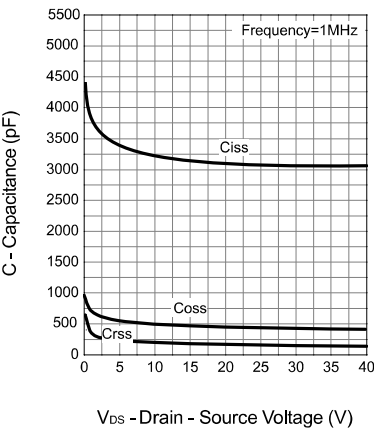
Capacitance
