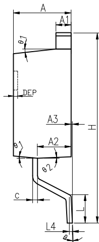
COMMON DIMENSIONS
