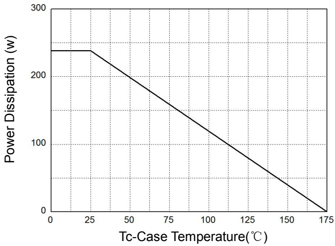
Figure 1: Power Dissipation
